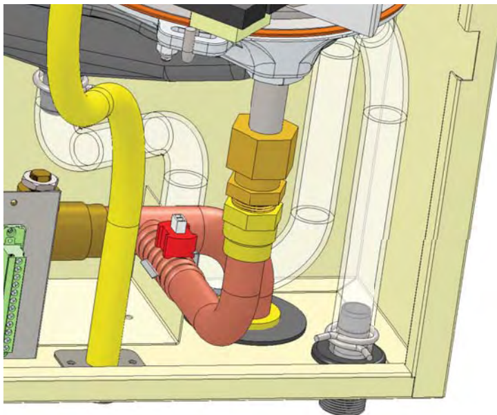
FIGURE 6-2 Safety Relief Valve Discharge Piping
